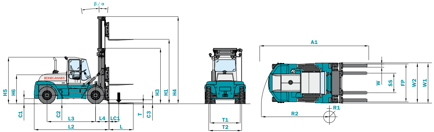
SMV 52-1200 B
