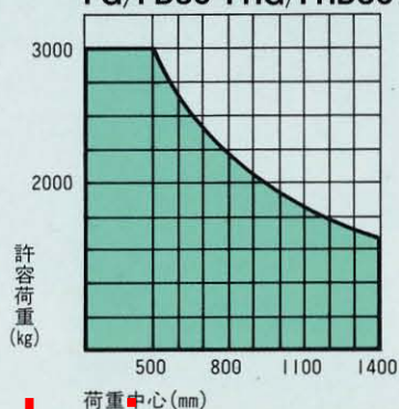
FG/FD30・FHG/FHD30
